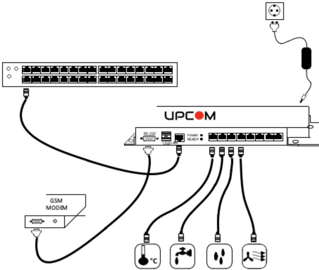
UP-Guard 6001 Main Unit connected to various sensors and GSM Modem.
