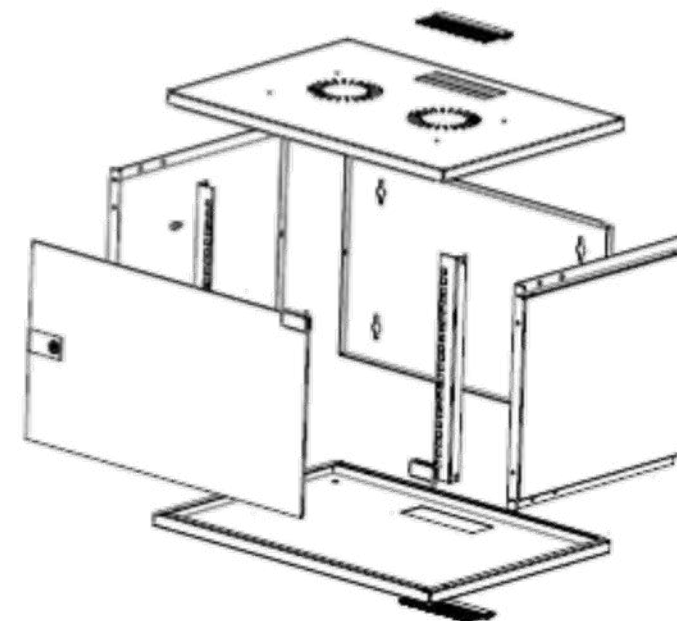
EXPLODED VIEW
