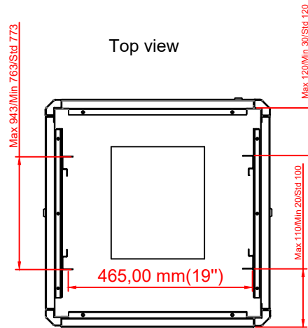
Max/std/min equipment mounting distance
