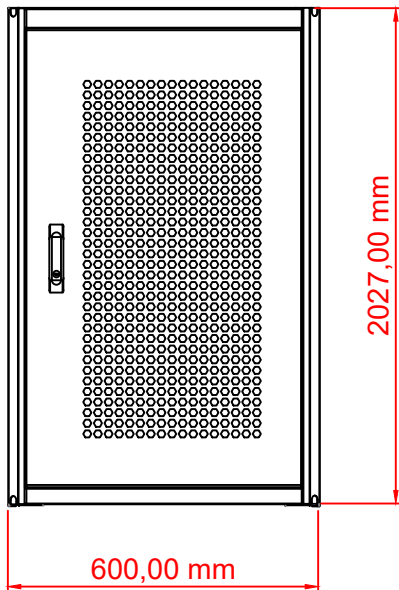
Rear view
