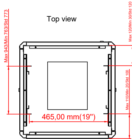
Max/std/min equipment mounting distance
