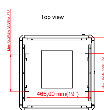
Max/std/min equipment mounting distance
