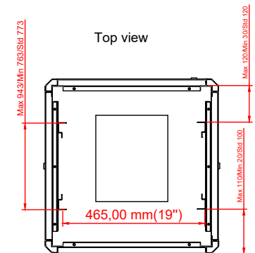
Max/std/min equipment mounting distance
