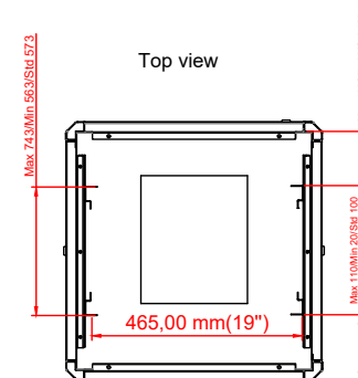
Max/std/min equipment mounting distance
