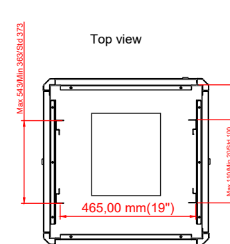
Max/std/min equipment mounting distance
