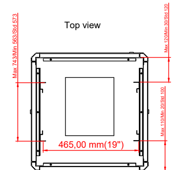
Max/std/min equipment mounting distance
