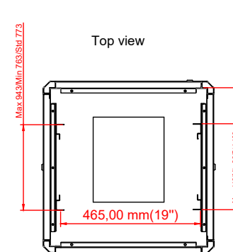
Max/std/min equipment mounting distance
